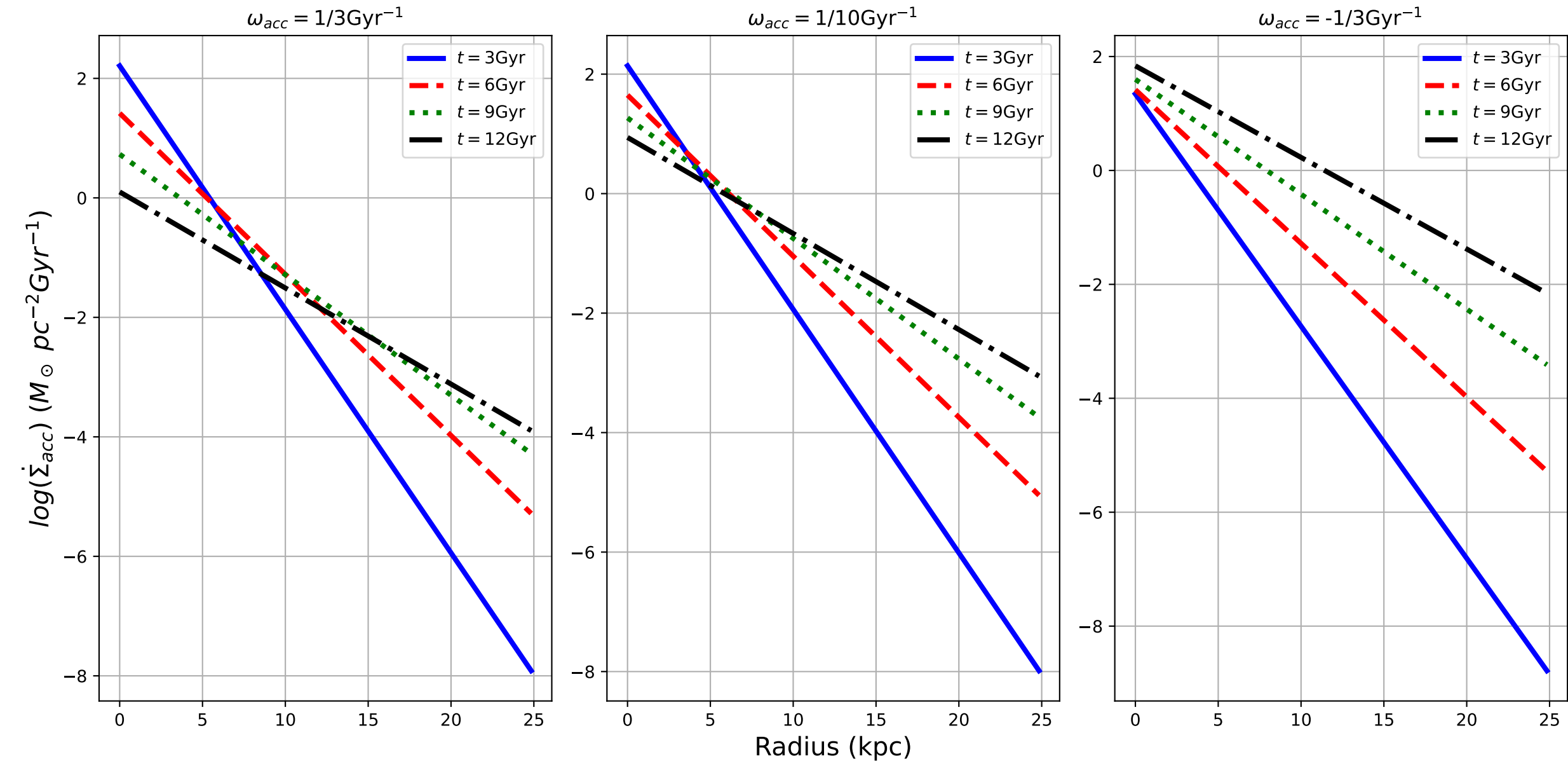
\dot{\Sigma}_{acc} vs r for different t and t_{acc}
